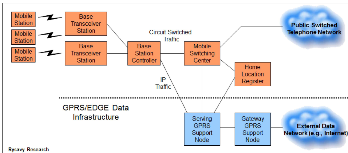
Figure 120: GSM/GPRS/EDGE Architecture
