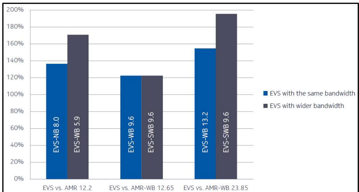
Figure 86: EVS Voice Capacity Compared to AMR and AMR-WB 203
