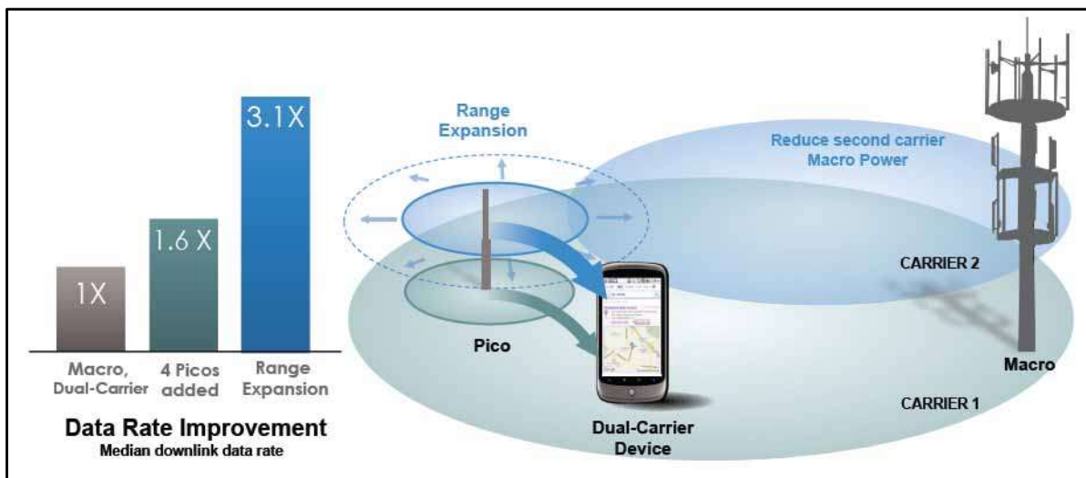
Figure 116: HSPA+ HetNet Using Multipoint Transmission 239
