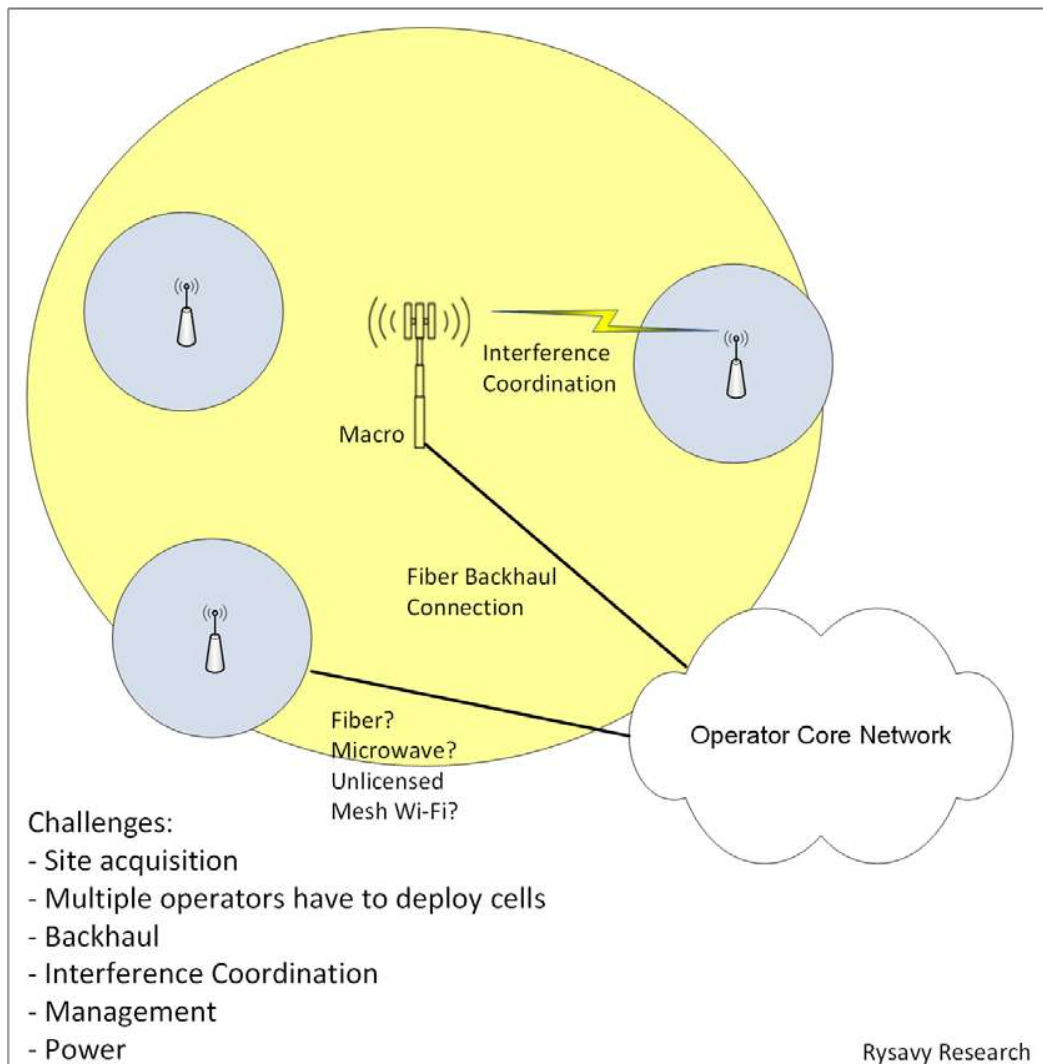
Figure 25: Small-Cell Challenges
