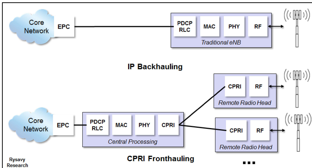
Figure 99: Potential Cloud RAN Approach
