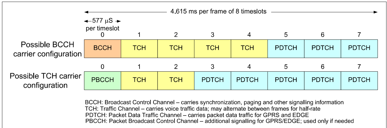
Figure 121: Example of GSM/EDGE Timeslot Structure 247
