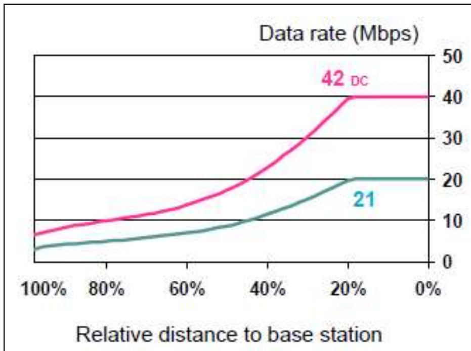
Figure 118: Dual-Carrier HSPA+ Throughputs 242
