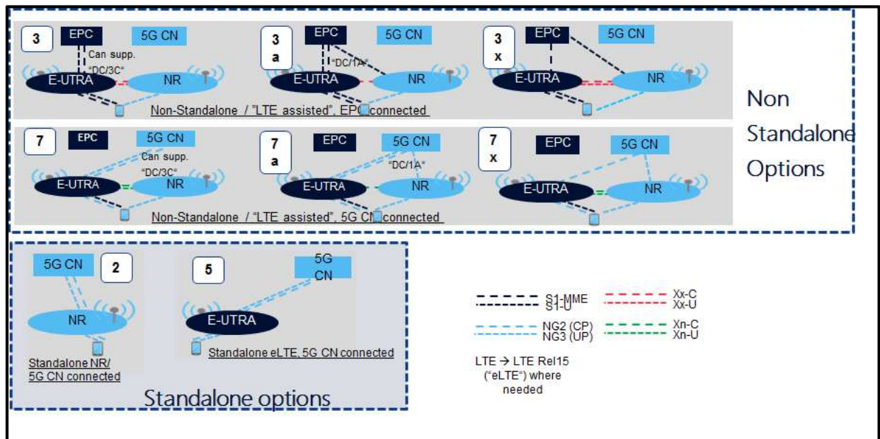
Figure 48: 5G Network Architecture Options in 3GPP Release 15 151
