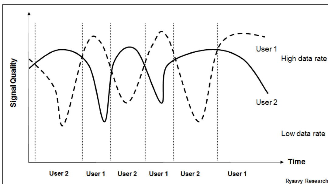
Figure 112: User Diversity
