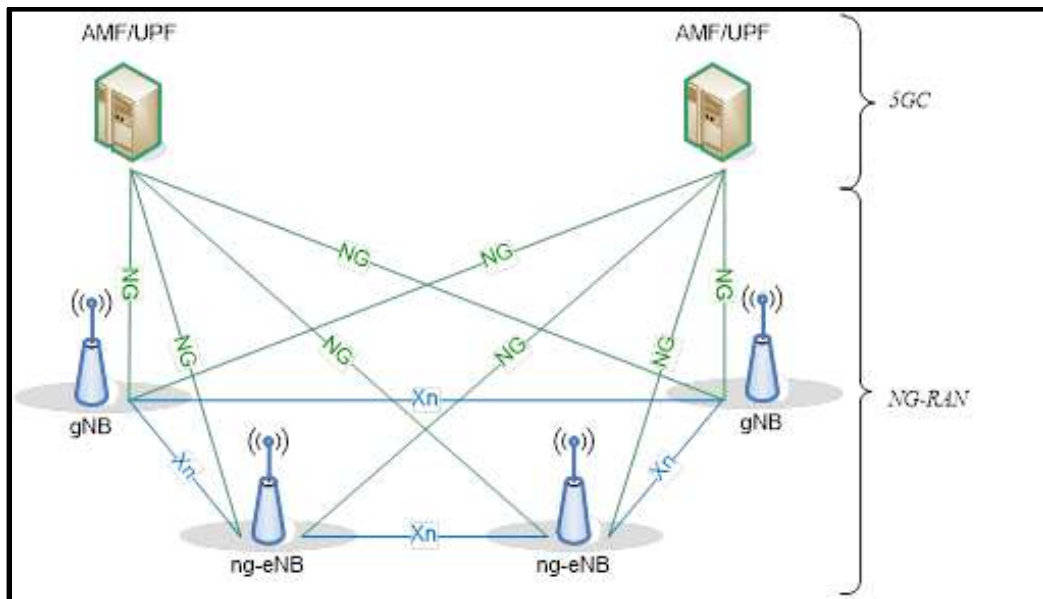
Figure 45: 5G Architecture 147
