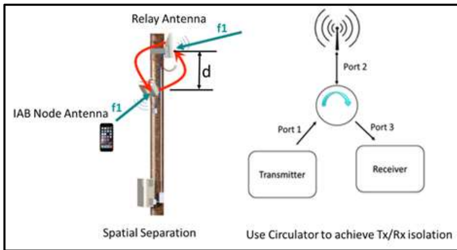
Figure 54: Antenna Separation to Reduce Interference
