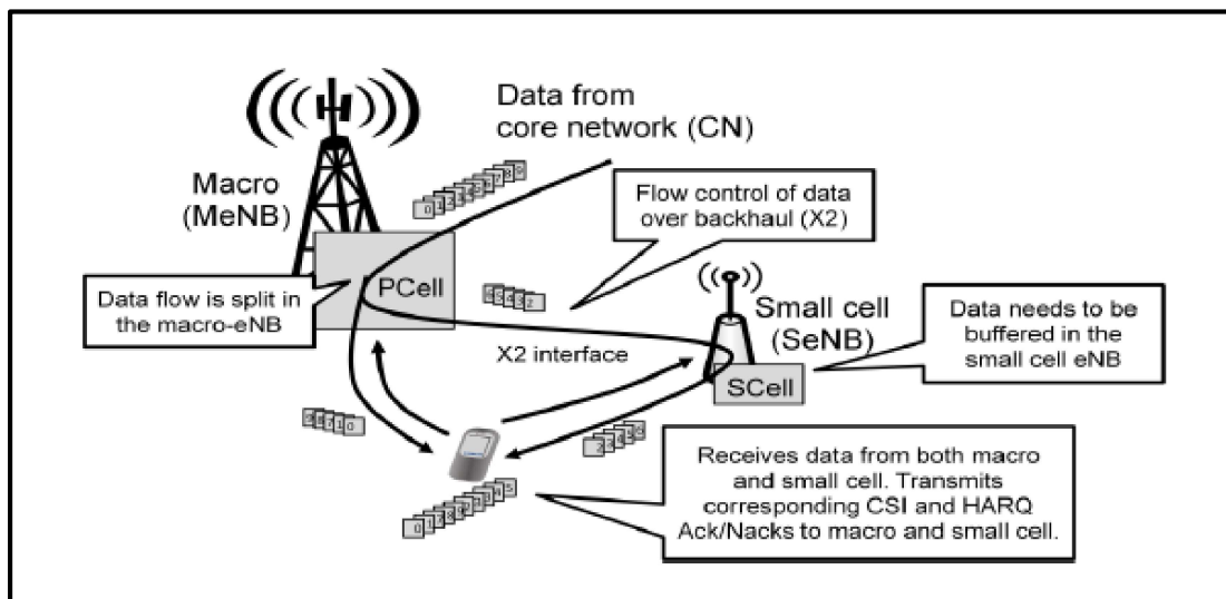
Figure 96: Dual Connectivity 214
