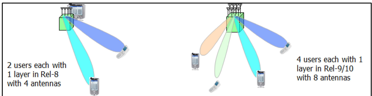
Figure 67: Multi-User MIMO 166
