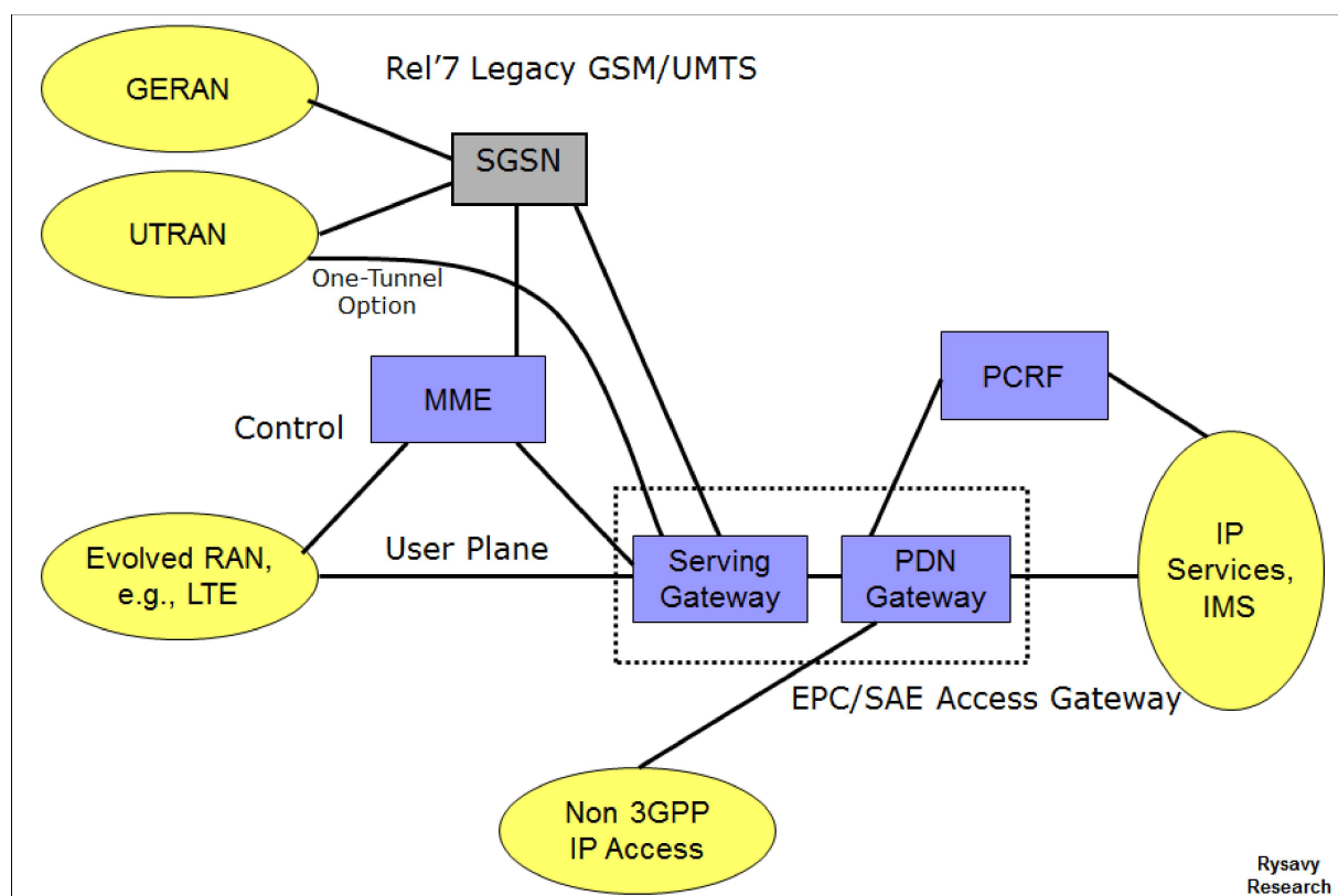
Figure 87: EPC Architecture
