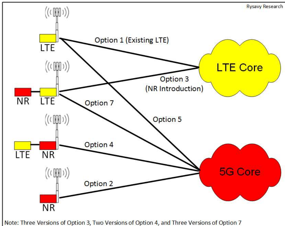
Figure 21: Release 15 Non-Standalone and Standalone Options
