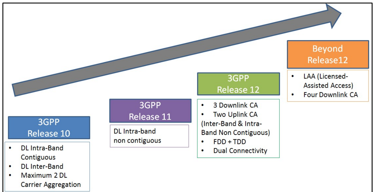
Figure 72: Carrier Aggregation Capabilities across 3GPP Releases 173
