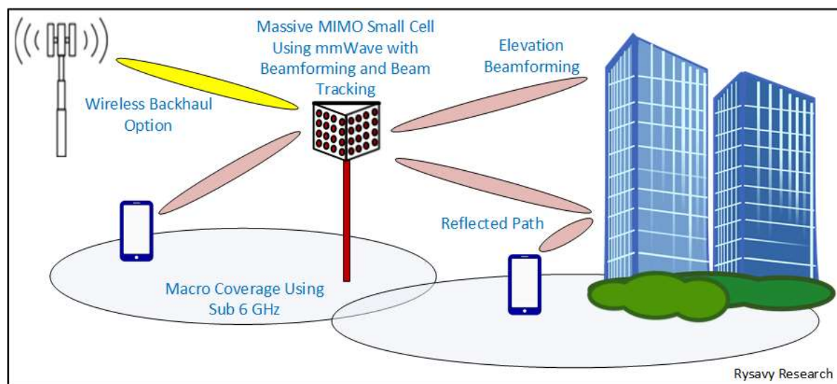
Figure 18: 5G Architecture for Low-Band/High-Band Integration
