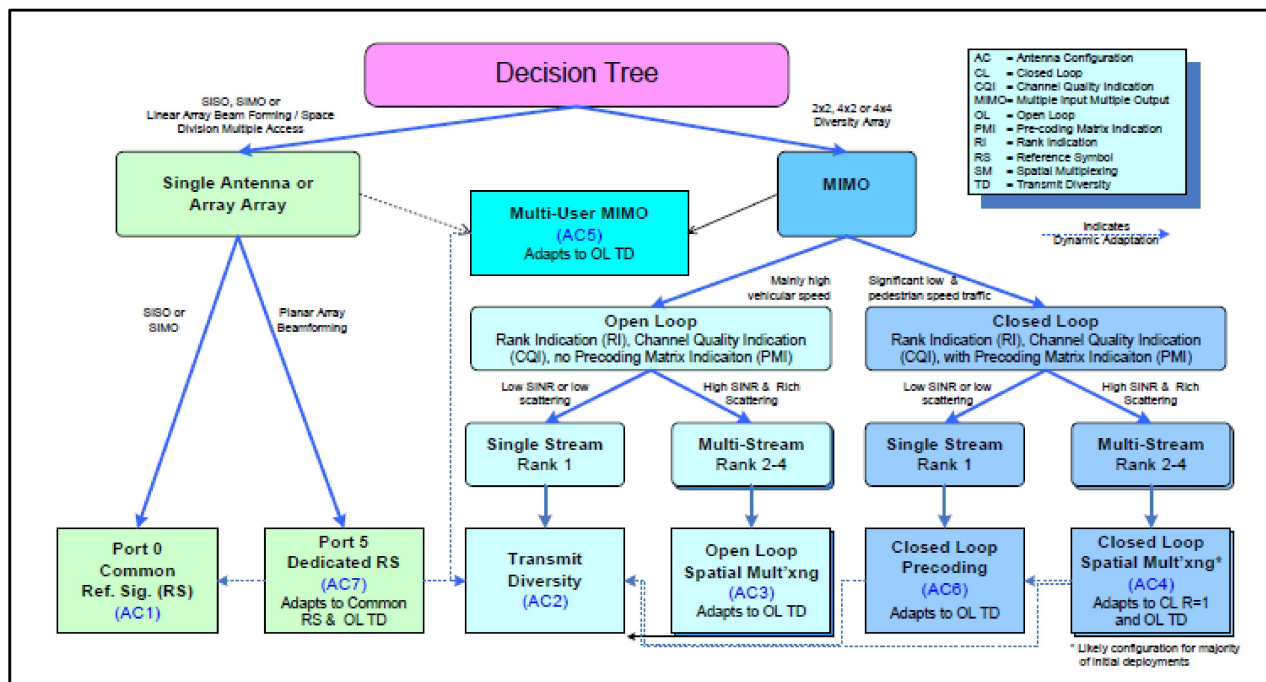
Figure 65: Decision Tree for Different Antenna Schemes 164
