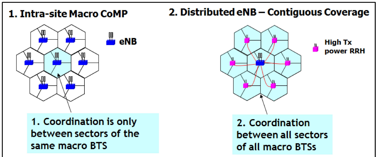
Figure 76: Different Coordination Levels for CoMP 177
