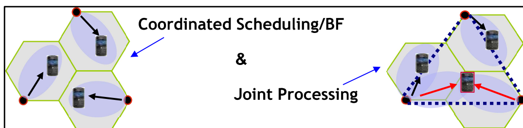
Figure 77: Coordinated Scheduling/BF and Joint Processing CoMP Approaches 178
