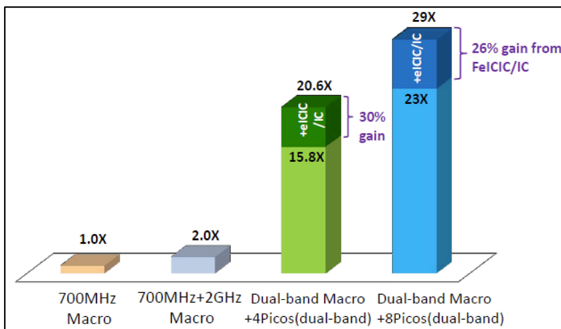
Figure 92: Median Throughput Gains in Hotspot Scenarios 209
