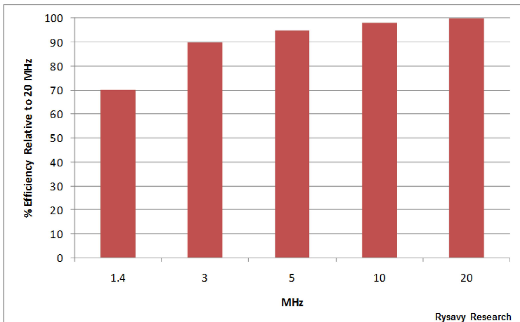
Figure 36: LTE Spectral Efficiency as Function of Radio Channel Size 111
