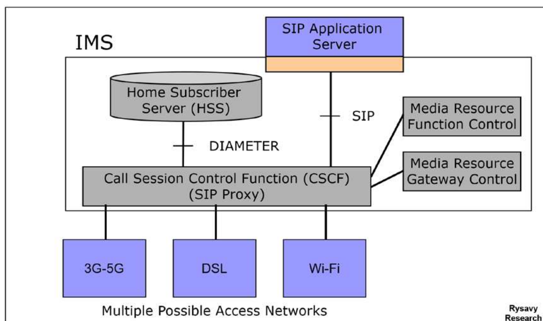
Figure 108: IP Multimedia Subsystem
