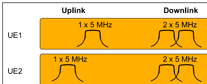
Figure 115: Dual-Carrier Operation with One Uplink Carrier 238
