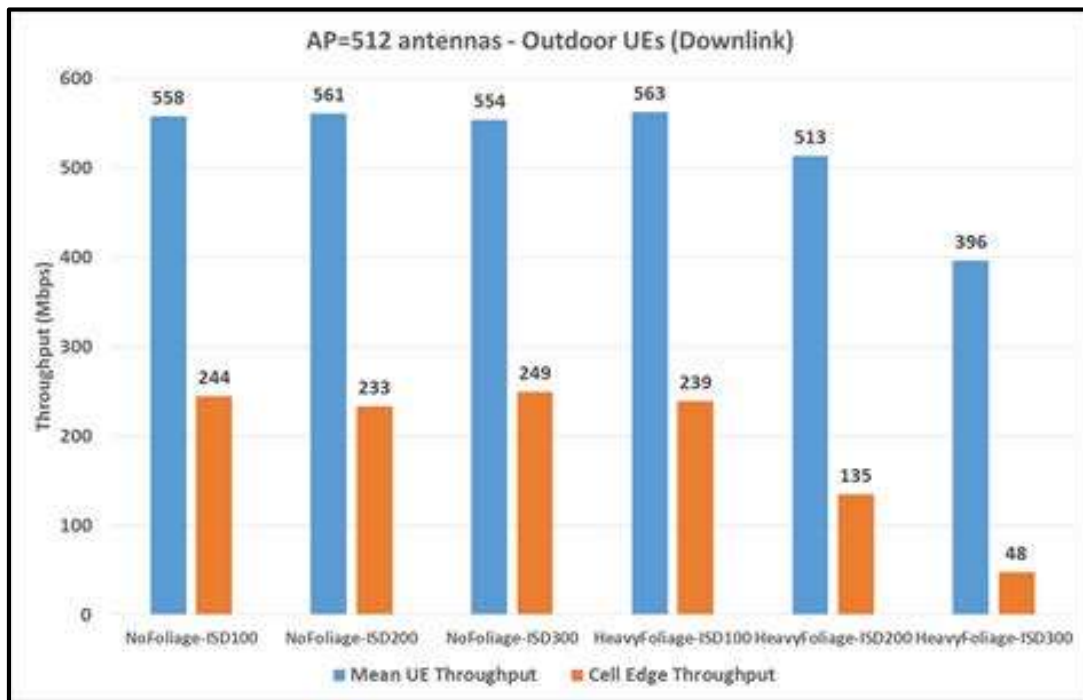
Figure 57: Downlink Performance, Different ISDs, Foliage vs. None 156
