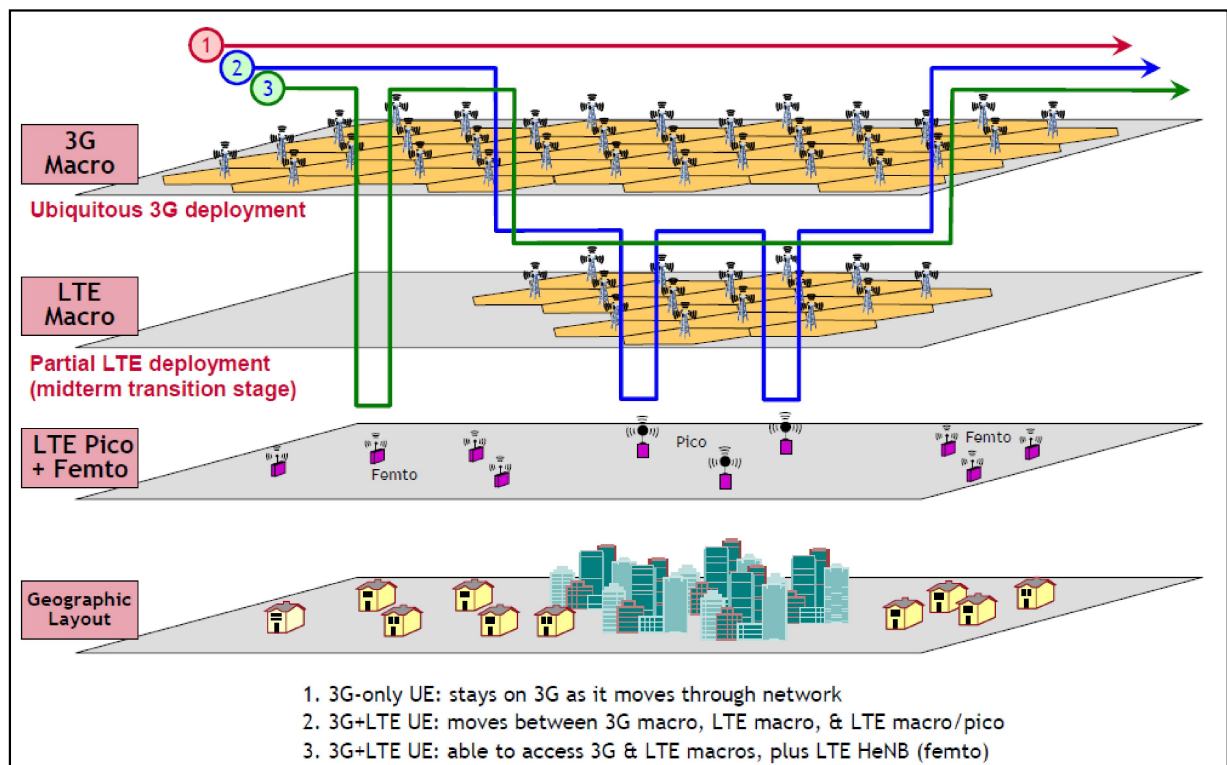
Figure 88: Load Balancing with Heterogeneous Networks 206
