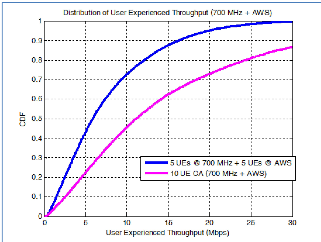
Figure 75: Gains from Carrier Aggregation 176
