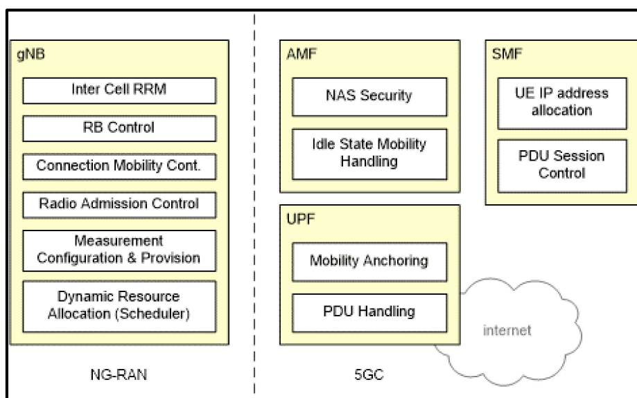
Figure 46: Functional Split between NG-RAN and 5GC 148
